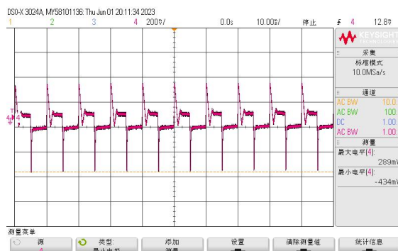
Vin=230VAC 10%-100%动态
