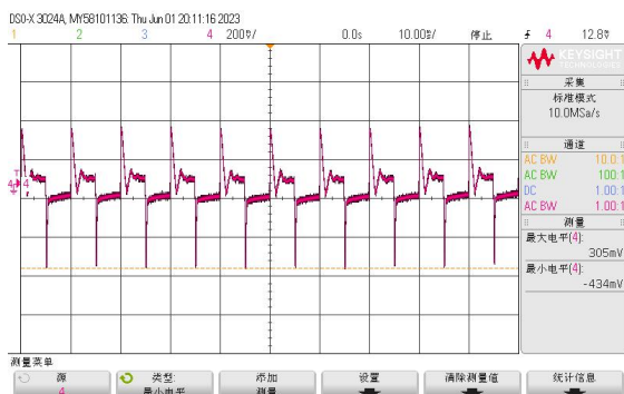
Vin=115VAC 10%-100%动态
