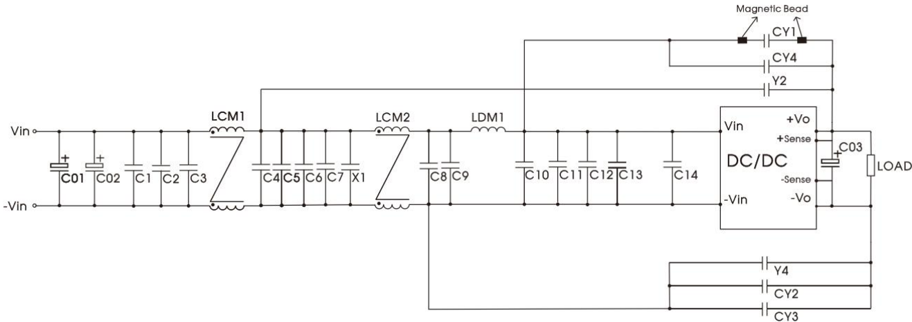
VCB4805/12SBO-100W(F)R3(-N)
